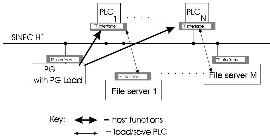
Fig. 5.3: Direction of the Host Functions in a Network
