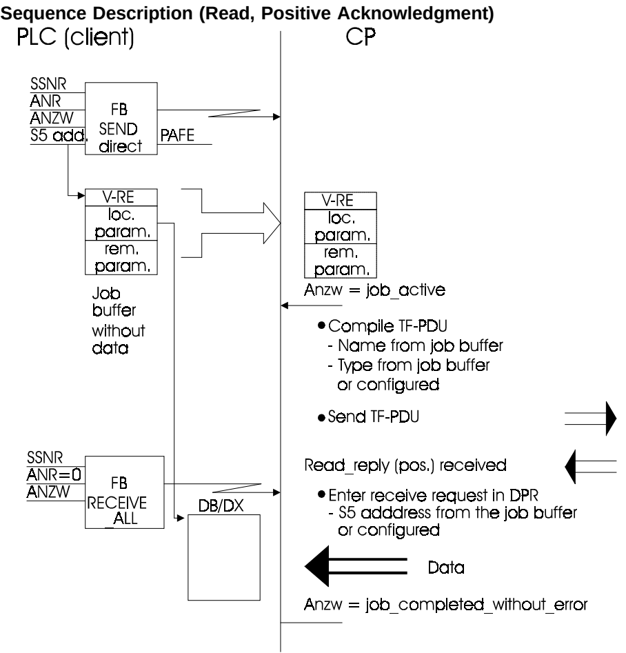
Fig. 7.4: Sequence Description (Read, Positive Acknowledgment)
