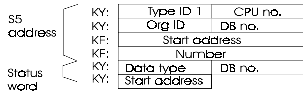
Fig. 7.16: S5-Specific Free Format Address in Job Buffer with Status Word
