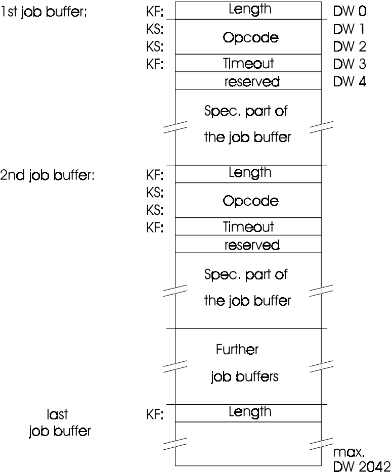
Fig. 6.1: Structure of a Data Block with Job Buffers
