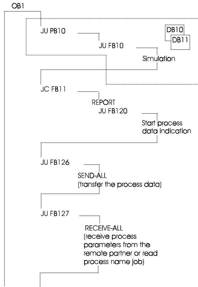
Fig. A.16: Program Structure of the PLC Programs on the Server PLC
