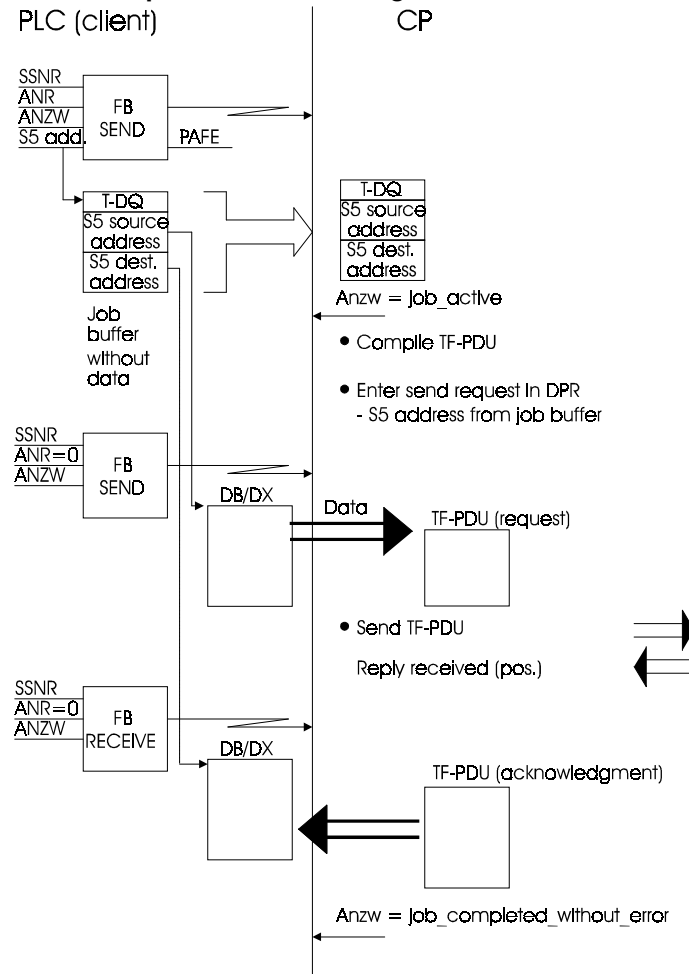
Fig. 10.11 Transparent Data Exchange with Source ID "DB" or "DX"
