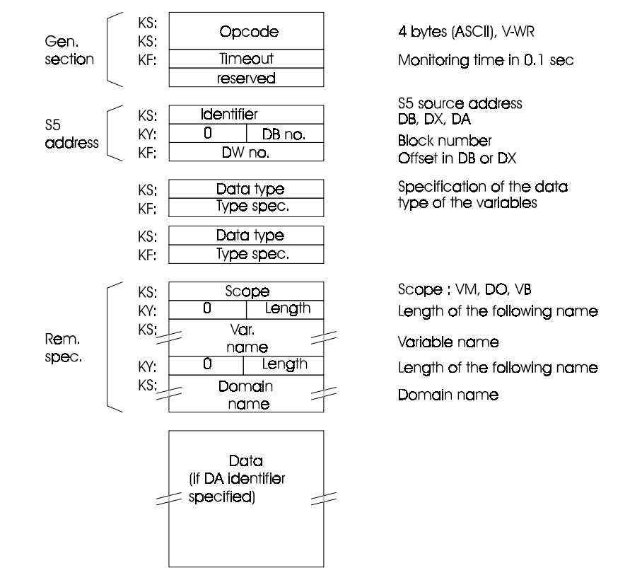
Fig. 7.6: Job Buffer for TF Variable Service "Write"
