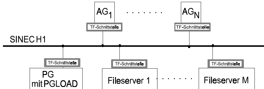
Fig. 5.1: Example of a Network when using PG Load
