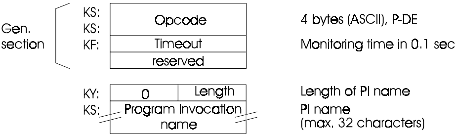
Fig. 8.25 Structure of the Job Buffer for TF Service "Delete Program Invocation"
