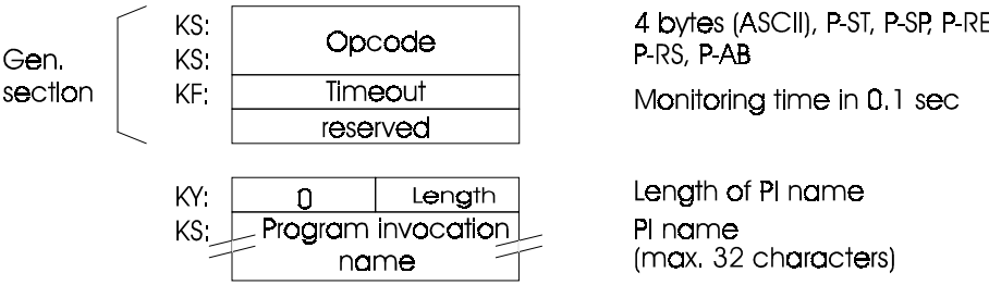
Fig. 8.28 Structure of the Job Buffer
