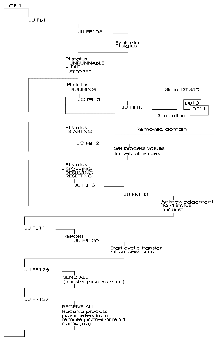
Fig. A.18 Taking the Domains out of the Original Program File of the Server PLC
