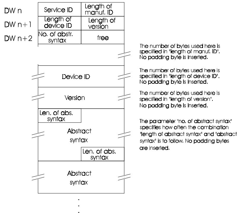
Fig. 9.5 Structure of the Reply Data in the Data Block
