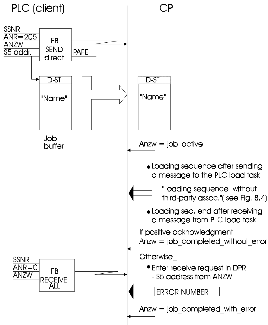
Fig. 8.12 Sequence 'Store Domain Content' (local PLC)
