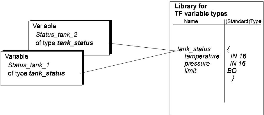
Fig. 4.2: Relationship Between TF Variables and TF Variable Types
