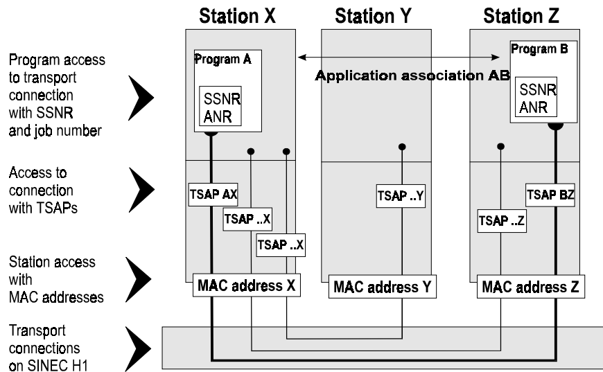
Fig. 2.3: Access by Application Associations to the Transport Services
