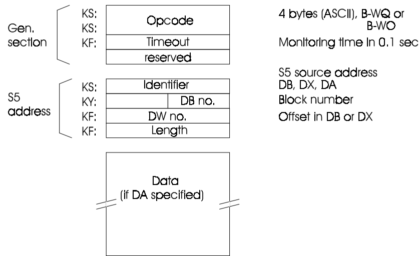
Fig. 10.3 Structure of the Job Buffer "Write Byte String"
