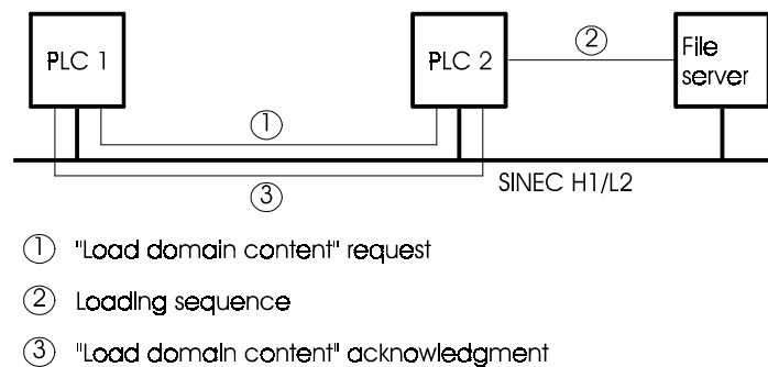
Fig. 8.2 Loading a Further PLC (third-party association)
