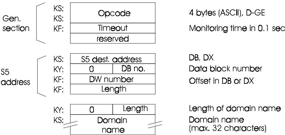
Fig. 8.15 Job Buffer "Get Domain Attributes"
