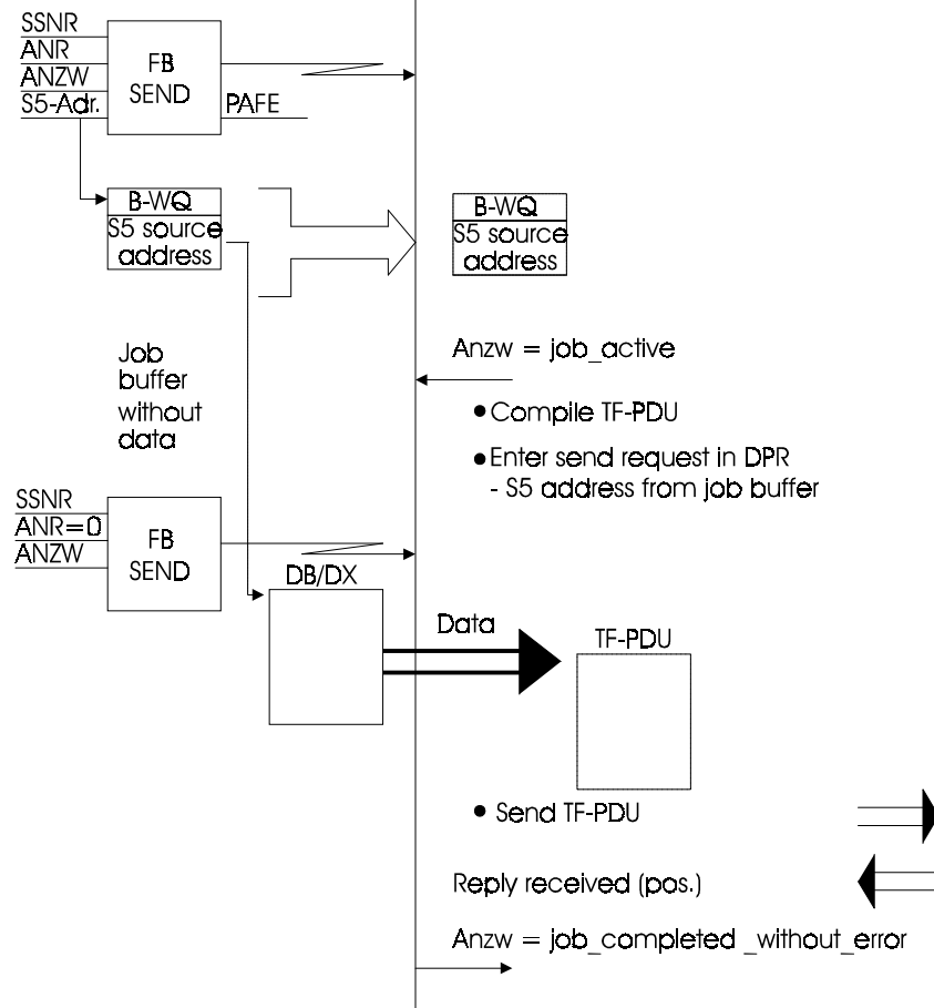
Fig. 10.4 Write Byte String with Acknowledgment (Example: Source ID = DA)
