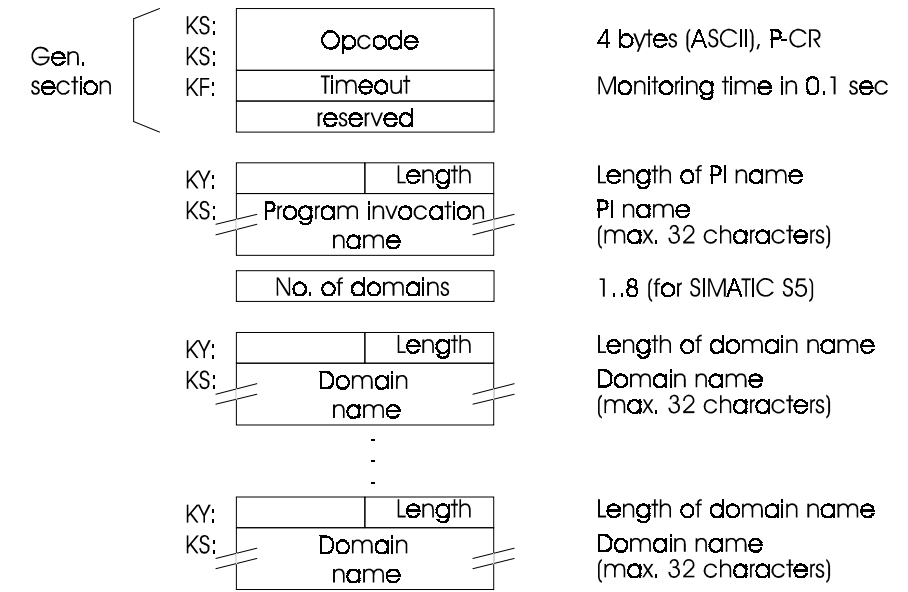
Fig. 8.22 Structure of the Job Buffer for TF Service "Create Program Invocation"
