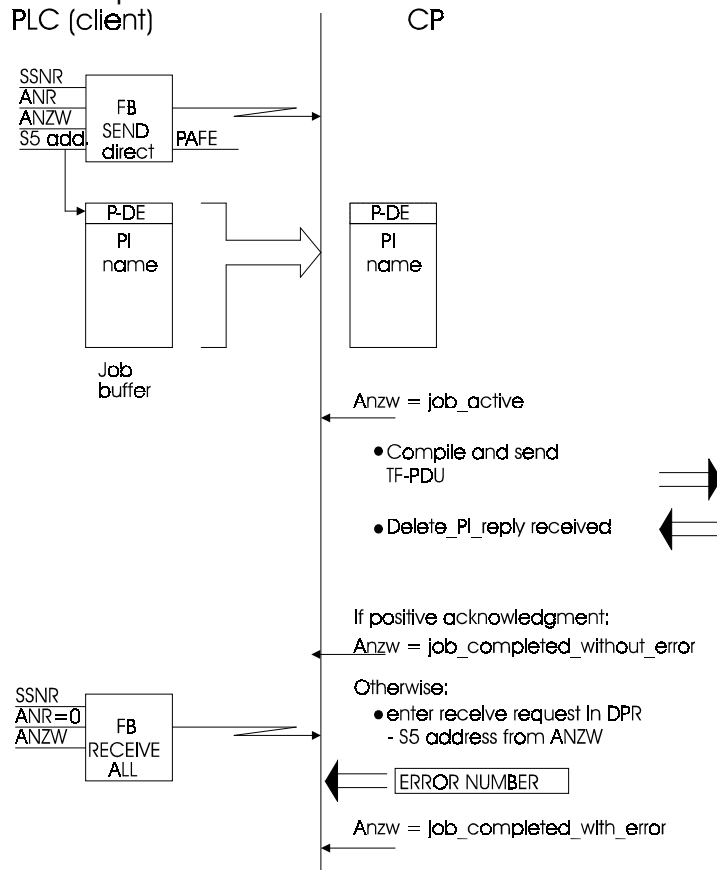
Fig. 8.26 Sequence 'Delete Program Invocation'
