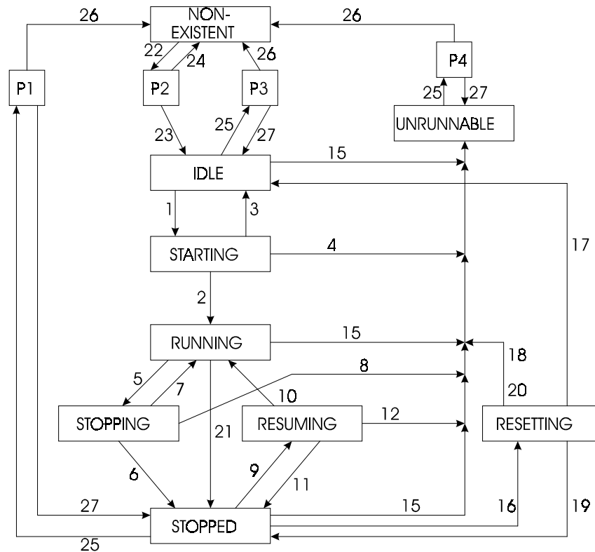
Fig. 8.19 Status Diagram of a Program Invocation
