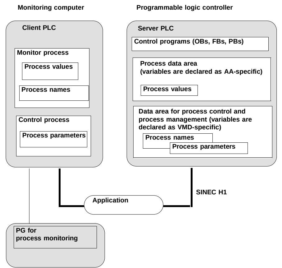
Fig. A.1: Example Configuration for Stage 1 - Variable Services
