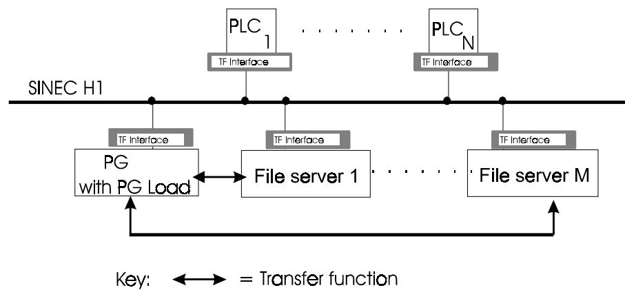
Fig. 5.2: Direction of the Transfer Functions in a Network
