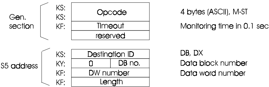
Fig. 9 - 1 Structure of the Job Buffer "VMD Status"
