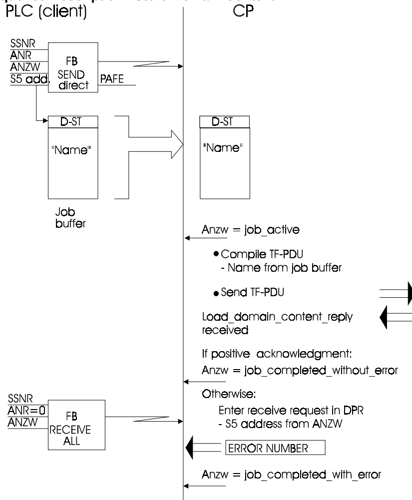
Fig. 8.11 Sequence 'Store Domain Content' (second PLC)
