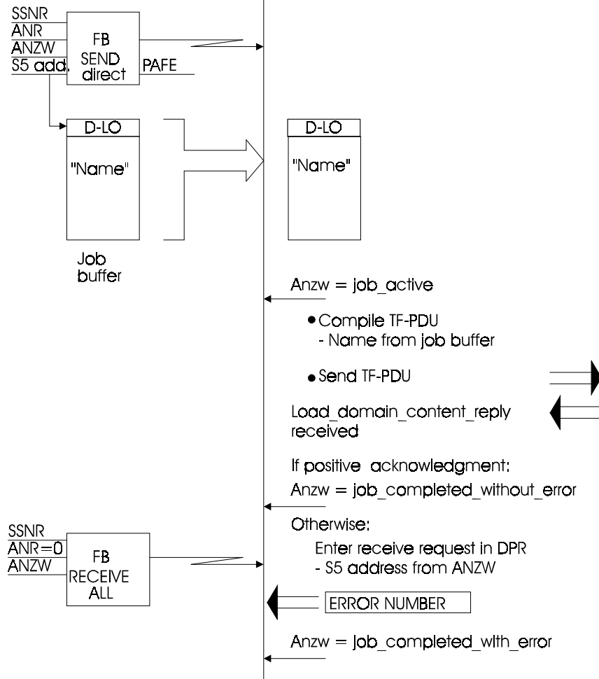
Fig. 8.7 Sequence "Load-Domain Content" (second PLC)
