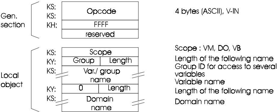
Fig. 7.10: Structure of the Job Buffer for TF Variable Service "Information Report"
