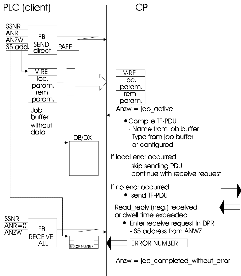
Fig. 7.5: Sequence Description (Read, Negative Acknowledgment)
