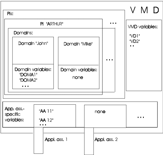
Fig. 7.1: Example of VMD Structure
