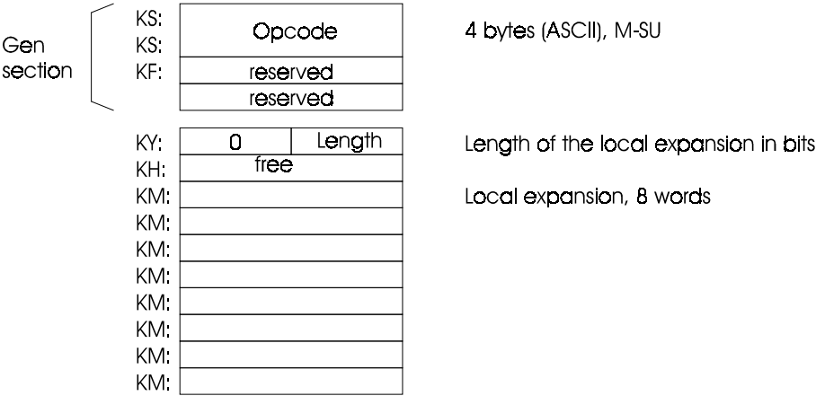
Fig. 9.3 Structure of the Job Buffer "Unsolicited Status"
