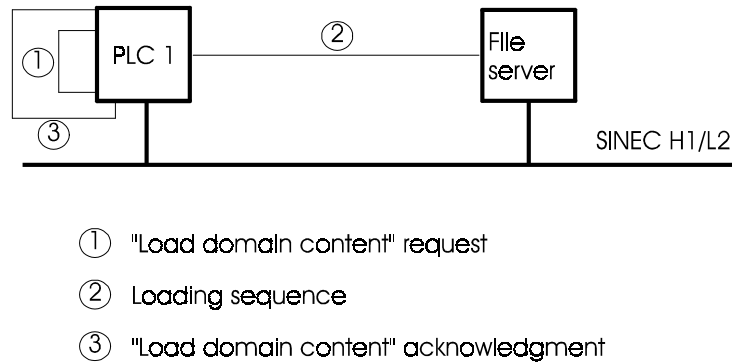
Fig. 8.1: Loading the Local PLC
