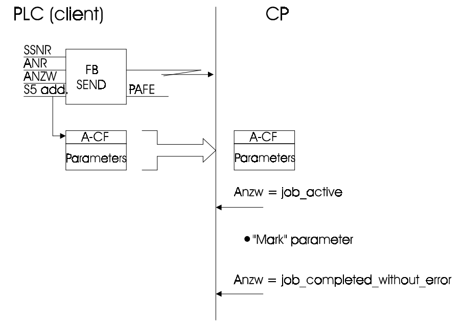
Fig. 9.7 Sequence: "Configure ANZW (local)"
