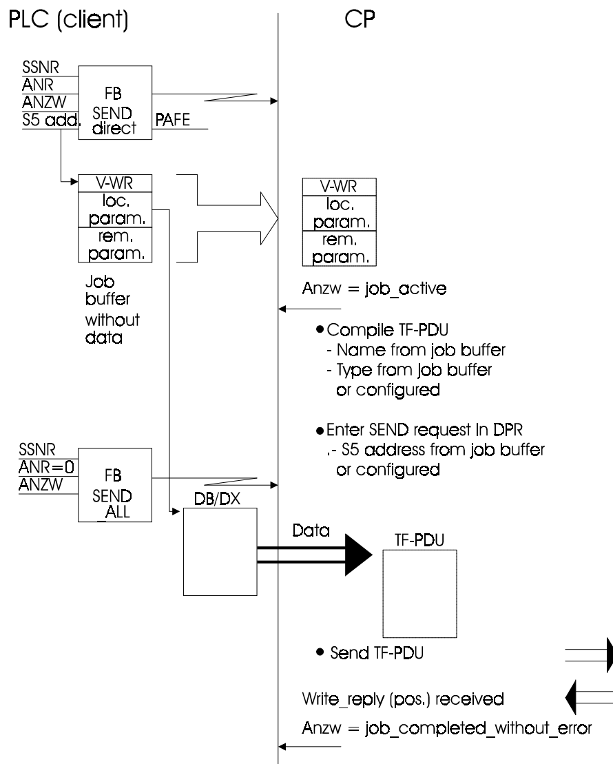
Fig. 7.7: Sequence Description Write with Source ID "DB" or "DX"
