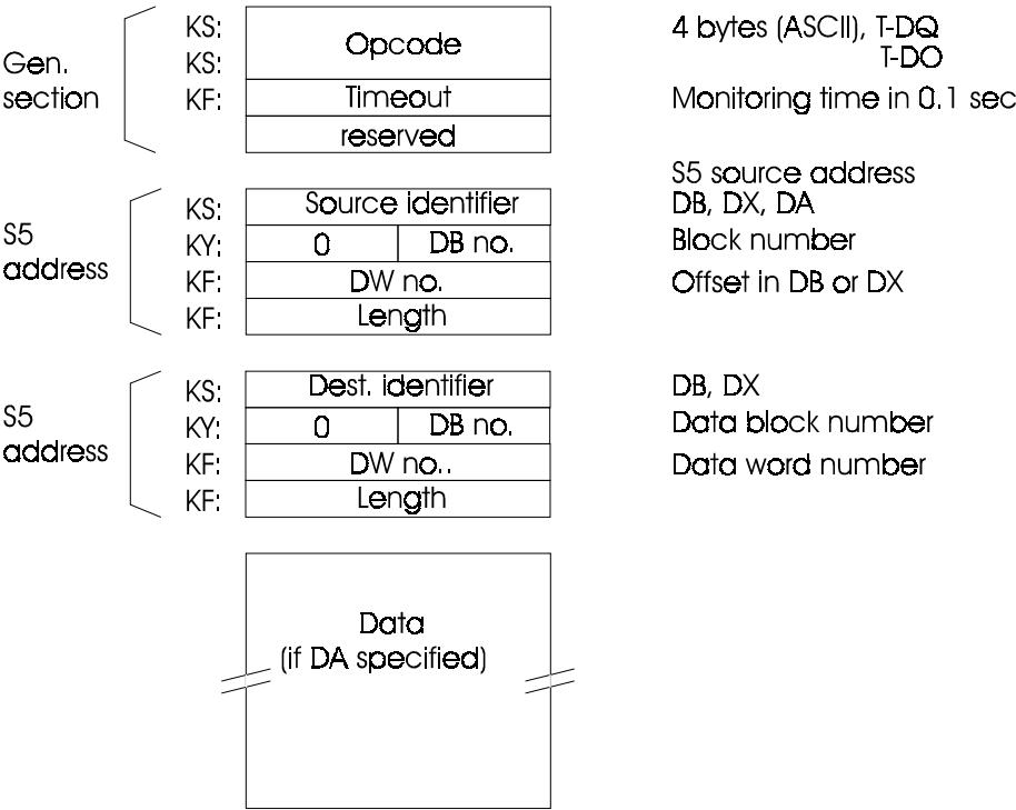
Fig. 10.10 Structure of the Job Buffer "Transparent Data Exchange"
