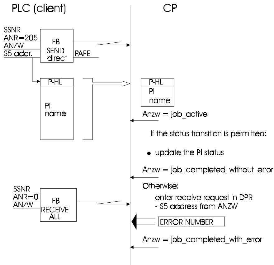
Fig. 8.29 Sequence "Local Program Stop"
