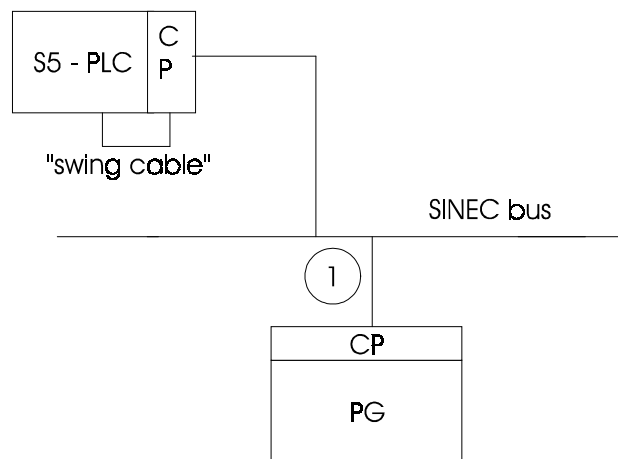
Fig. 2.6: Domain Services with the PG - 'Download/Upload'
