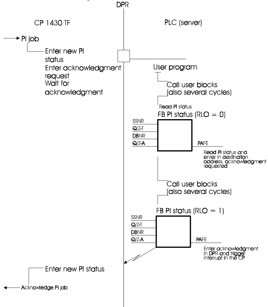
Fig. 8.20 General Sequence (no error) of a Status Change
