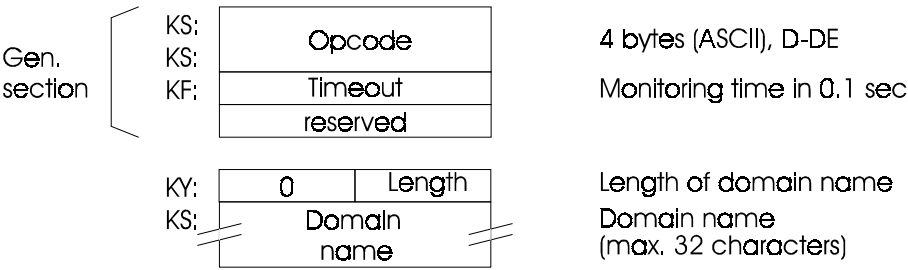
Fig. 8.13 Structure of the Job Buffer "Delete Domain"
