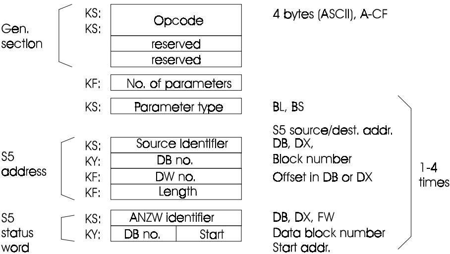
Fig. 10.8 Structure of the Job Buffer "Configure ANZW"
