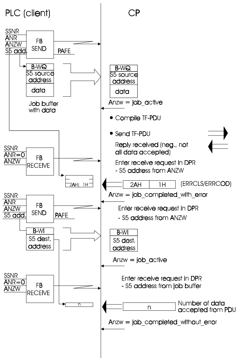
Fig. 10.7 Write Byte String with Ack. if Error Occurs, (Example: Source ID = DA)
