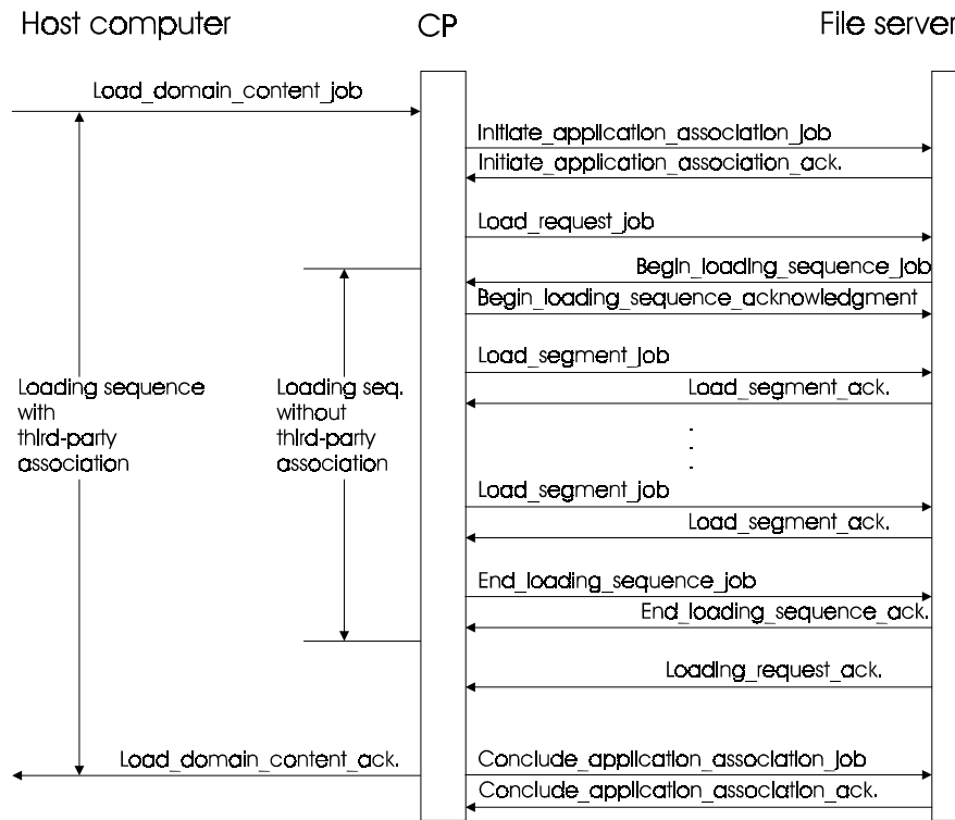
Fig. 8.3 Load Sequence with/without Third-Party Association
