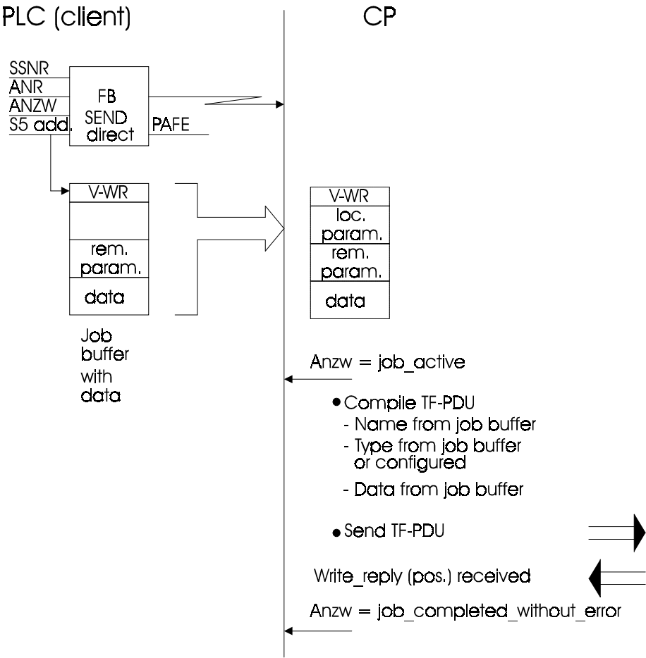
Fig. 7.8: Sequence Description Write with Source ID "DA"
