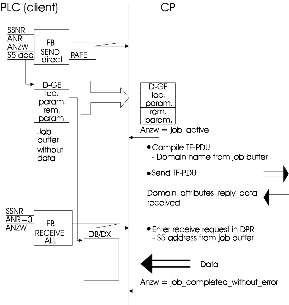
Fig. 8.16 Sequence Description (Get Domain Attributes, Positive Acknowledgment)
