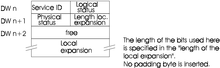
Fig. 9 - 2 Structure of the Reply Data in the Data Block
