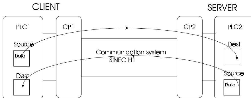
Fig. A.23: Transparent Data Exchange with Acknowledgment
