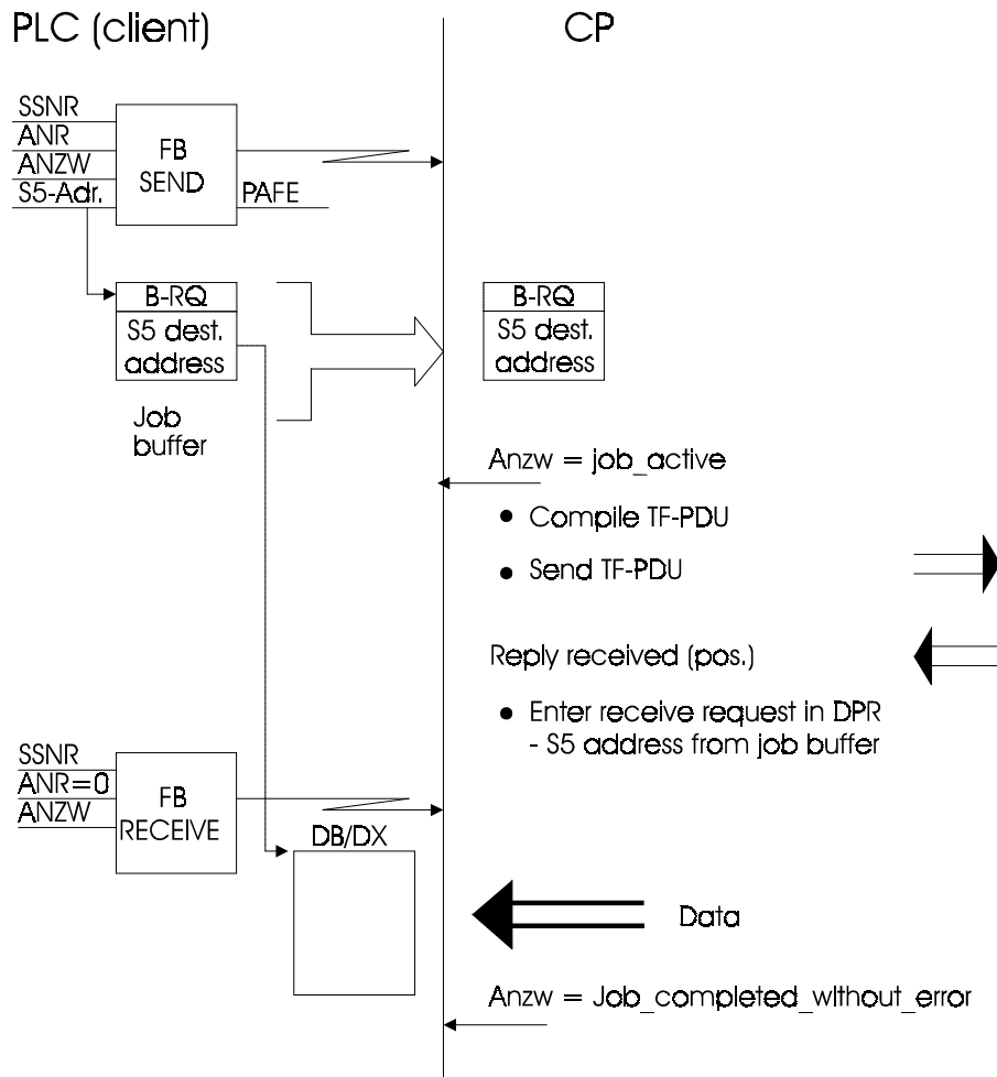
Fig. 10.2 Sequence "Read Byte String"
