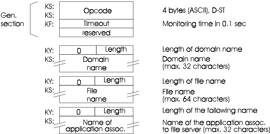
Fig. 8.10 Structure of the Job Buffer for TF Service "Store Domain Content"
